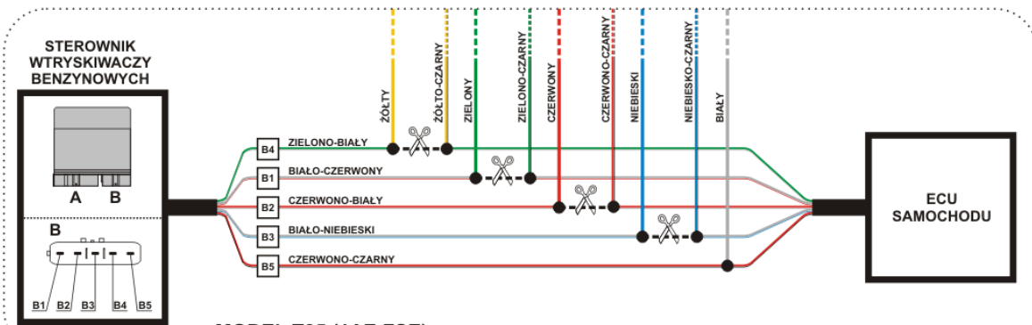
MODEL T25 (1AZ-FSE)
